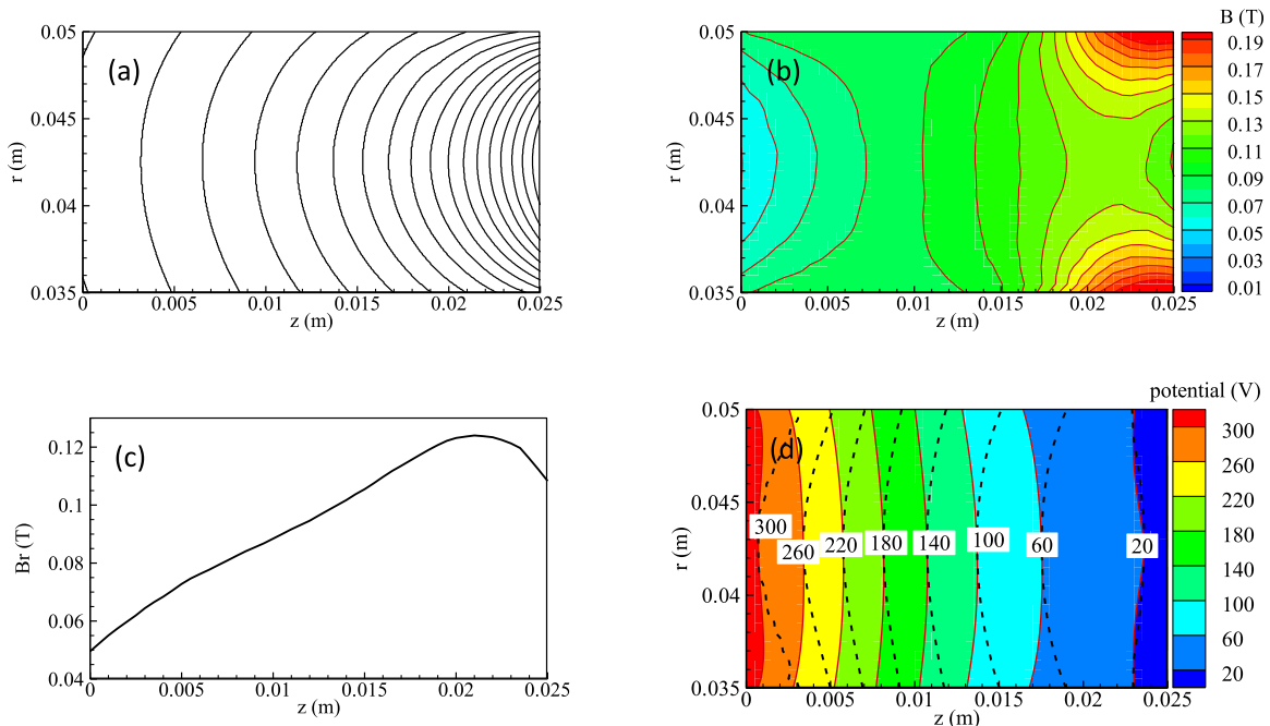
FIG. 3. Magnetic field and plasma potential distribution (Case 1): (a) magnetic field lines (Case 1), (b) magnetic field strength (unit: T), (c) B_r along the channel centerline (Case 1), (d) comparison of equipotential contours of plasma potential with “thermalized potential” (black dashed lines).
