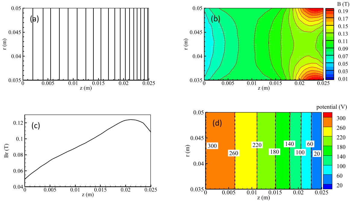
FIG. 2. Magnetic field and plasma potential distribution: (a) magnetic field lines, (b) magnetic field strength (unit: T), (c) B_r along the channel centerline, (d) comparison of equipotential contours of plasma potential with “thermalized potential” (black dashed lines).
